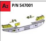
A2 P/N 547001 ATL HD bumper
