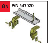
A3 P/N 547020 Winch mounting plate for original winch mount
